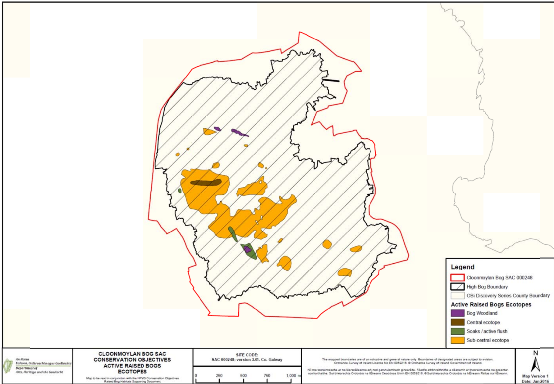
Map 2: Distribution of raised bog ecotopes on Cloonmoylan Bog.
