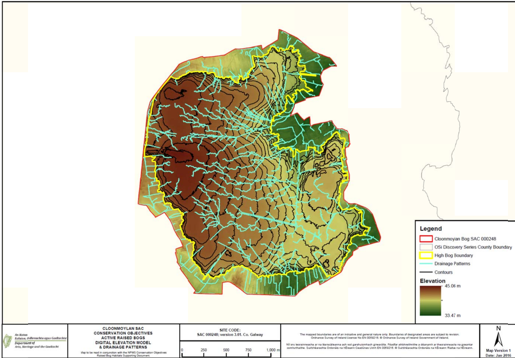
Map 3: Digital elevation model and drainage patterns at Cloonmoylan Bog.
