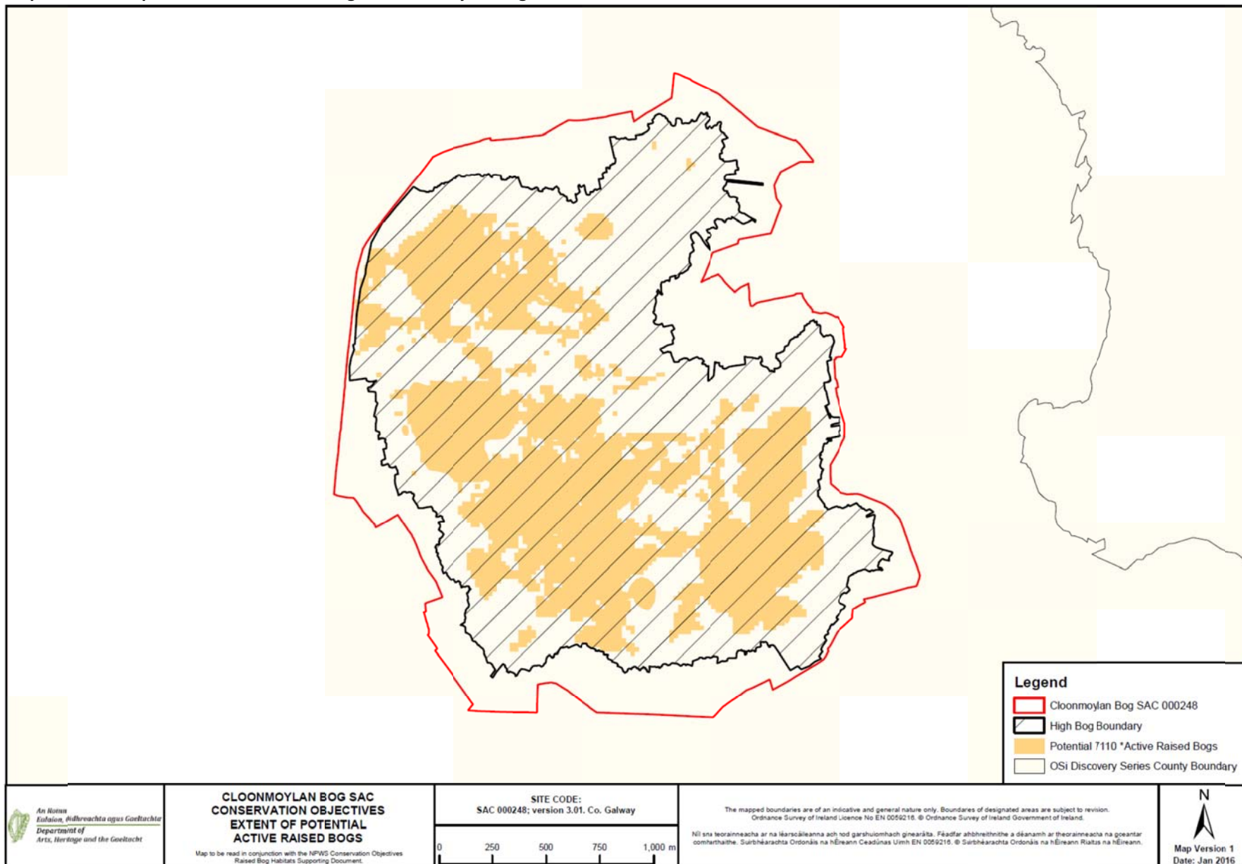
Map 1: Extent of potential active raised bog on Cloonmoylan Bog.
